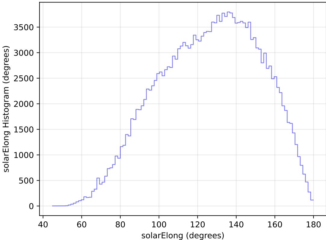
too_elab_r16_d2_griz_v3.4_10yrs WFD g band: solarElong Histogram
