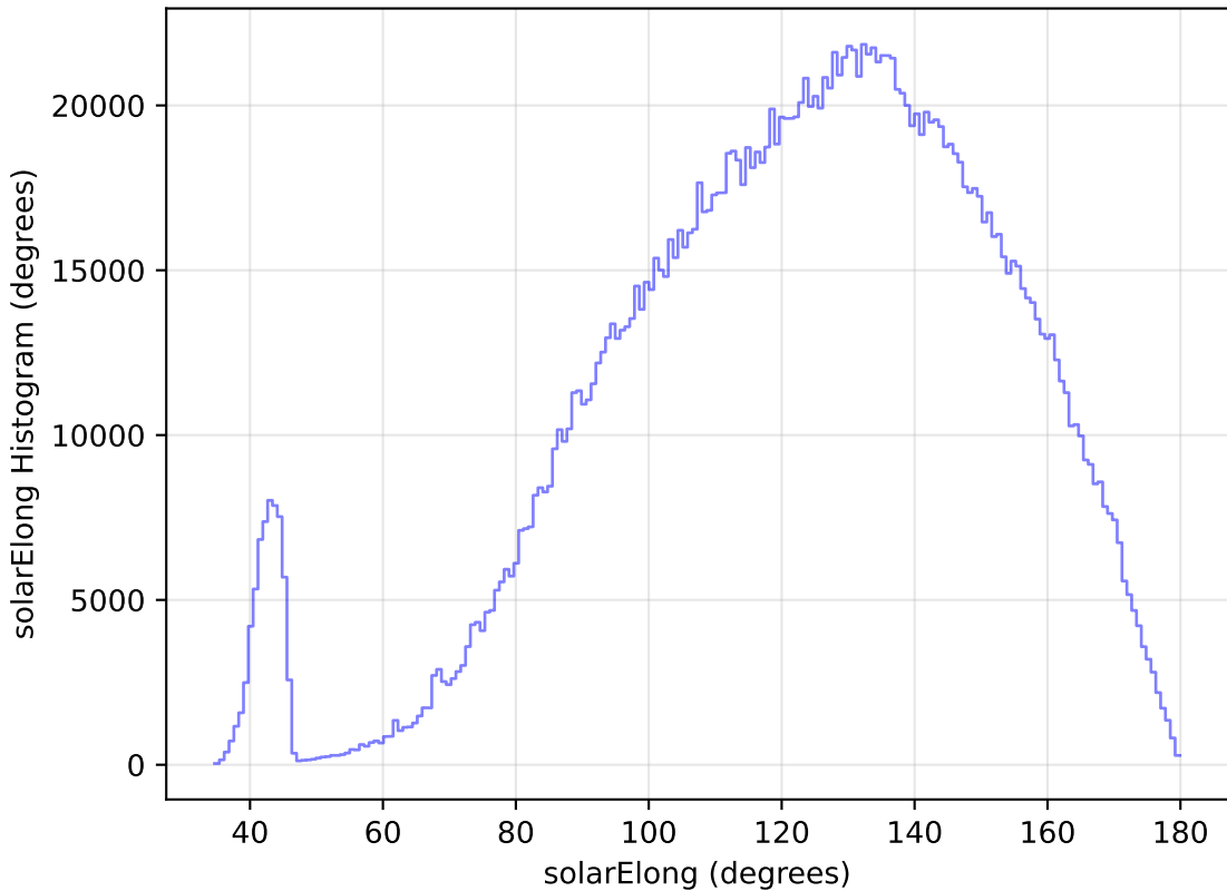
too_elab_r16_d2_griz_v3.4_10yrs WFD all bands: solarElong Histogram
