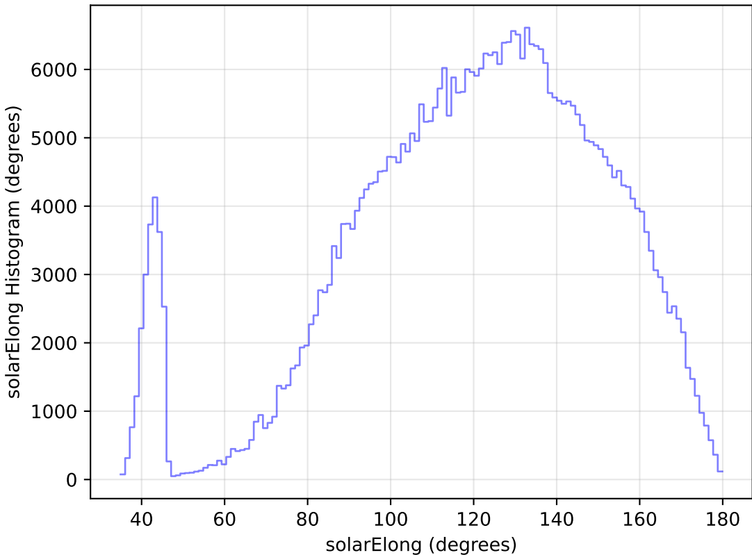
too_elab_r16_d2_griz_v3.4_10yrs All sky z band: solarElong Histogram
