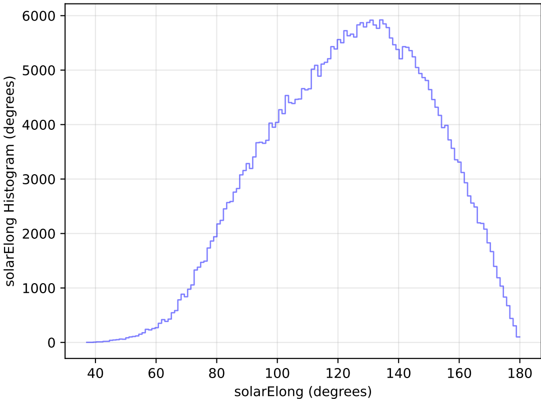
too_elab_r16_d2_griz_v3.4_10yrs All sky y band: solarElong Histogram
