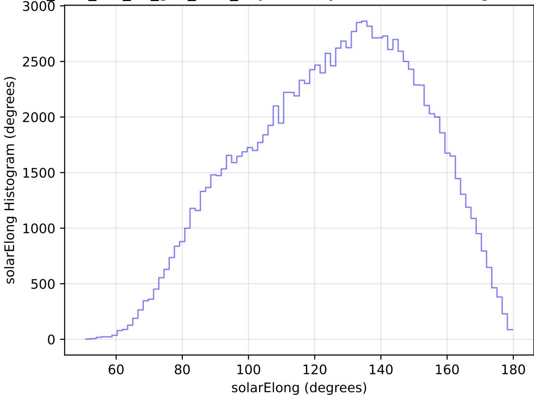
too_elab_r16_d2_griz_v3.4_10yrs All sky u band: solarElong Histogram
