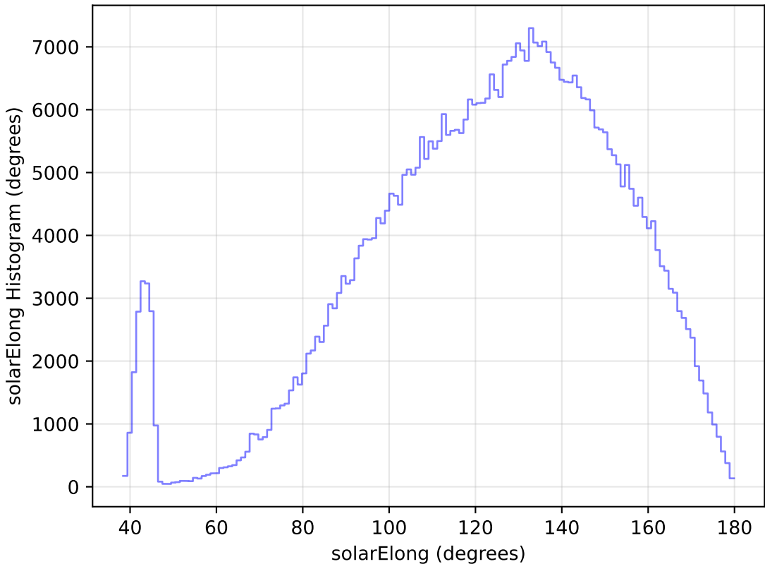
too_elab_r16_d2_griz_v3.4_10yrs All sky r band: solarElong Histogram
