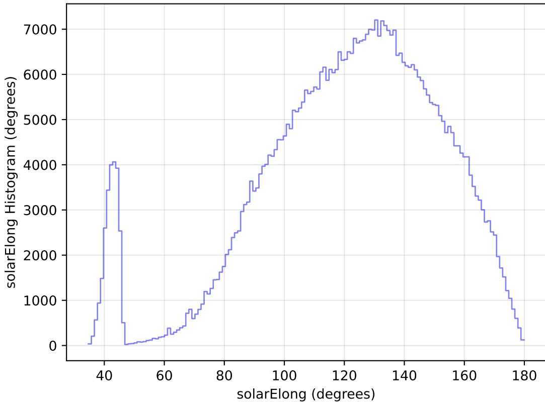
too_elab_r16_d2_griz_v3.4_10yrs All sky i band: solarElong Histogram
