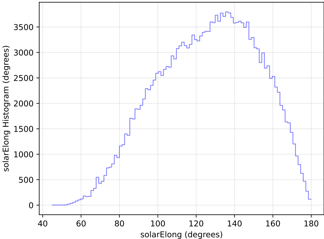
too_elab_r16_d2_griz_v3.4_10yrs All sky g band: solarElong Histogram
