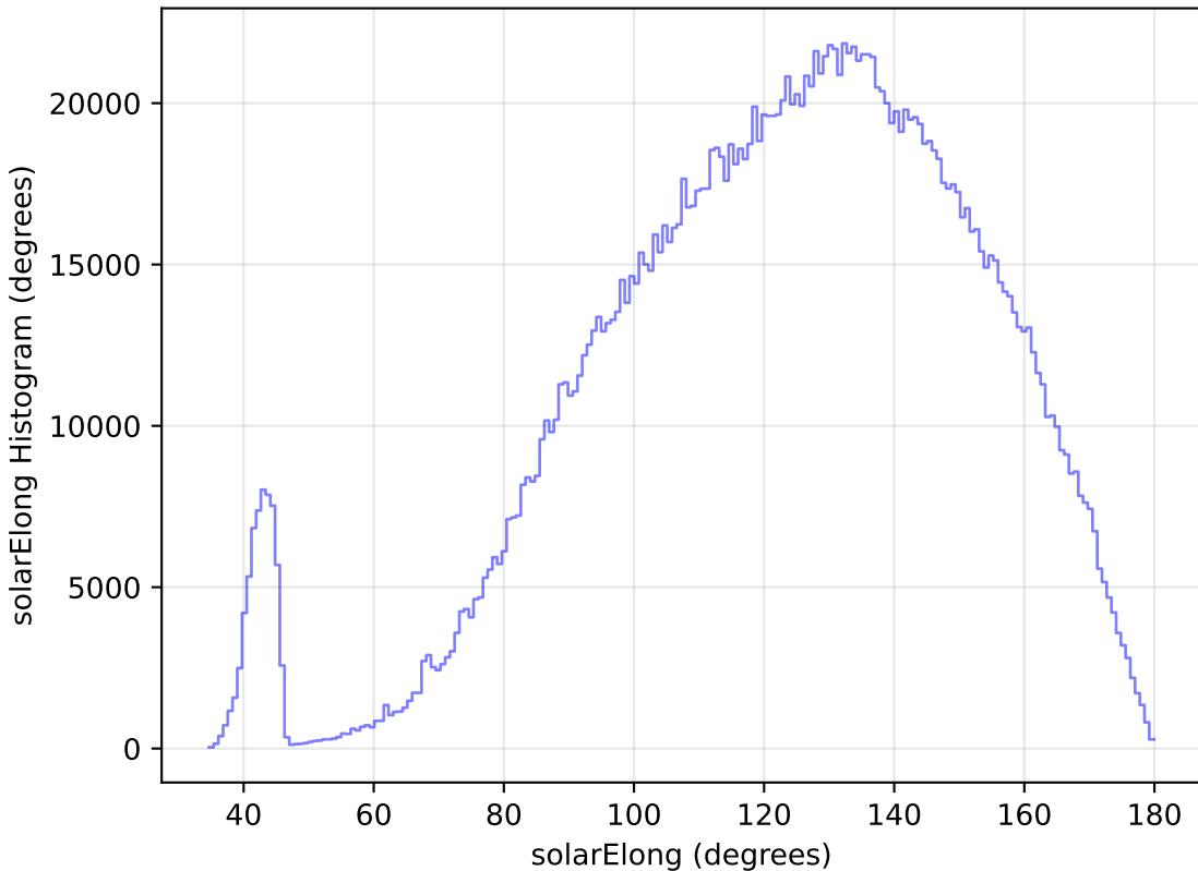
too_elab_r16_d2_griz_v3.4_10yrs All sky all bands: solarElong Histogram
