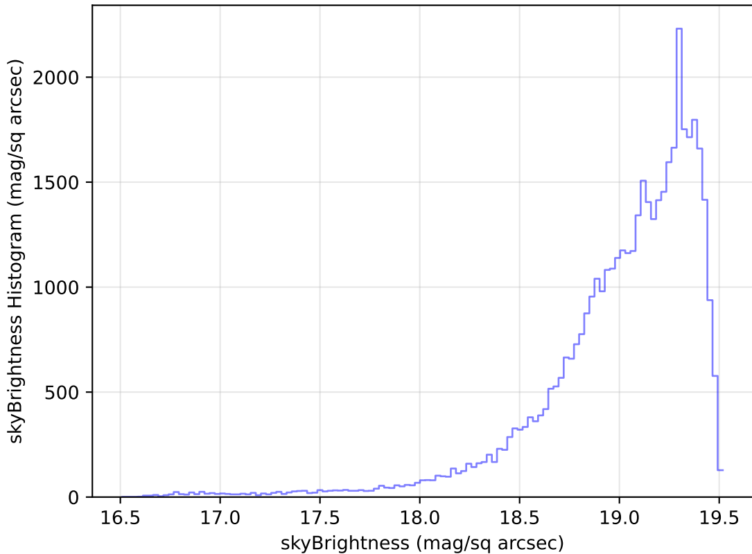
too_elab_r16_d2_griz_v3.4_10yrs Yr 1 z band: skyBrightness Histogram
