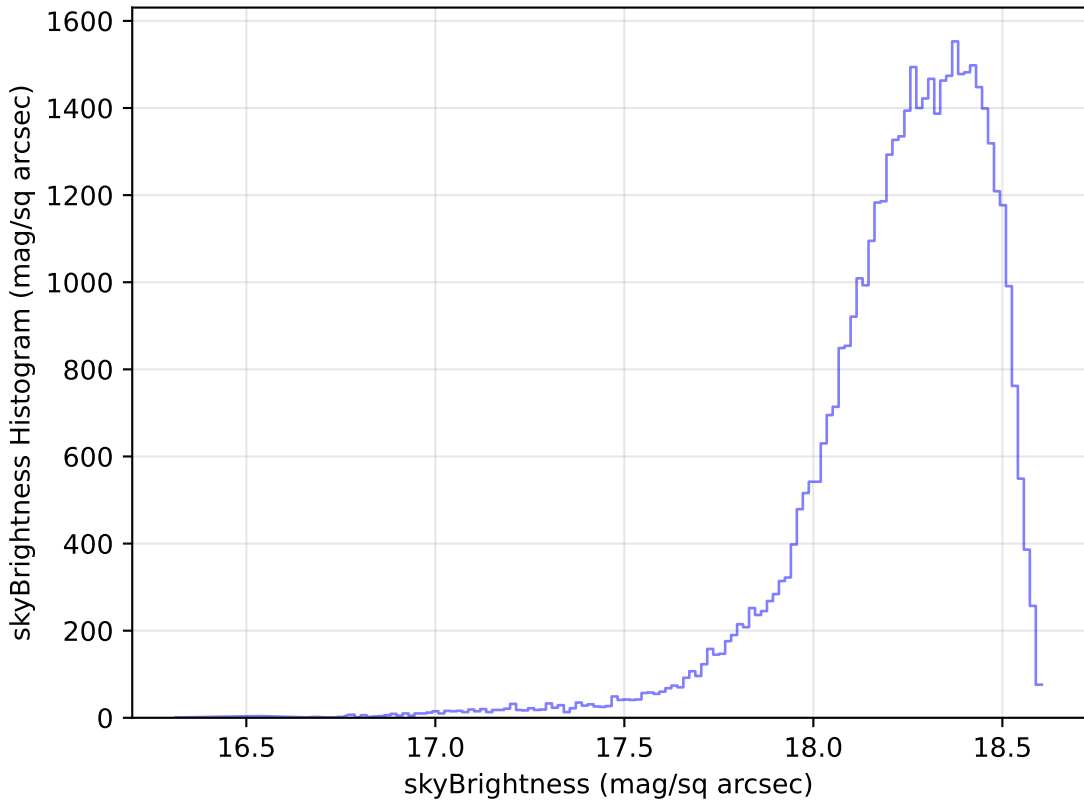
too_elab_r16_d2_griz_v3.4_10yrs Yr 1 y band: skyBrightness Histogram
