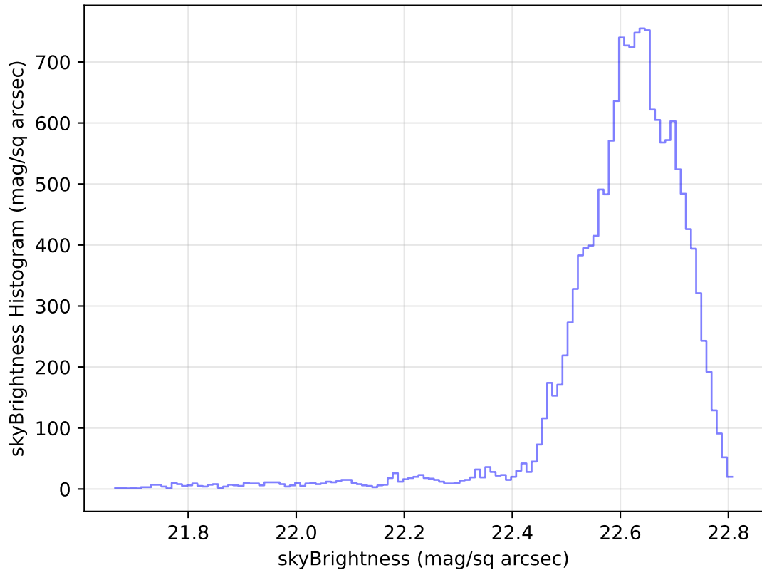
too_elab_r16_d2_griz_v3.4_10yrs Yr 1 u band: skyBrightness Histogram
