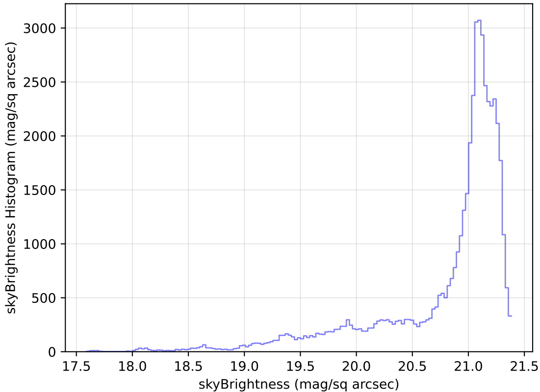
too_elab_r16_d2_griz_v3.4_10yrs Yr 1 r band: skyBrightness Histogram
