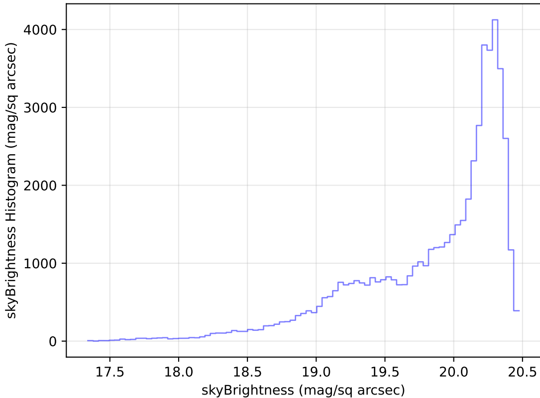
too_elab_r16_d2_griz_v3.4_10yrs Yr 1 i band: skyBrightness Histogram
