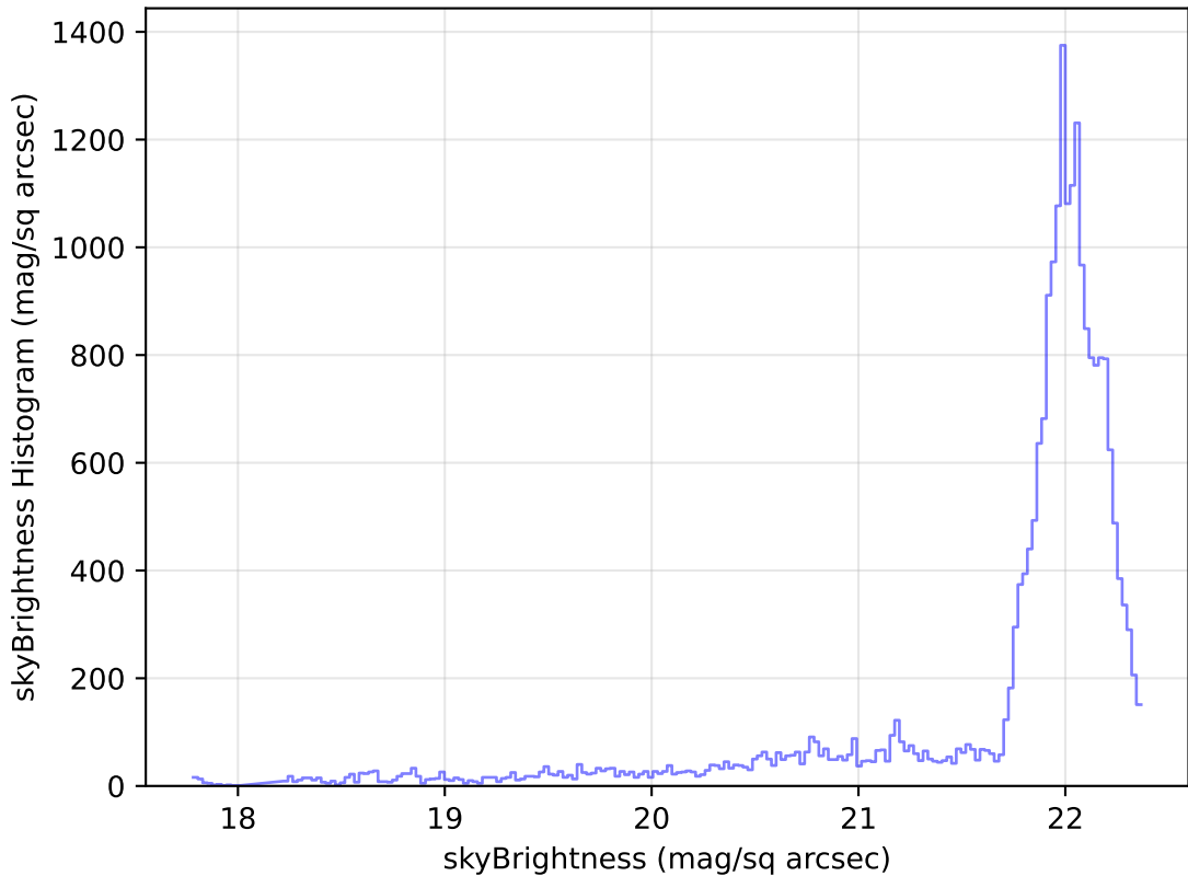
too_elab_r16_d2_griz_v3.4_10yrs Yr 1 g band: skyBrightness Histogram
