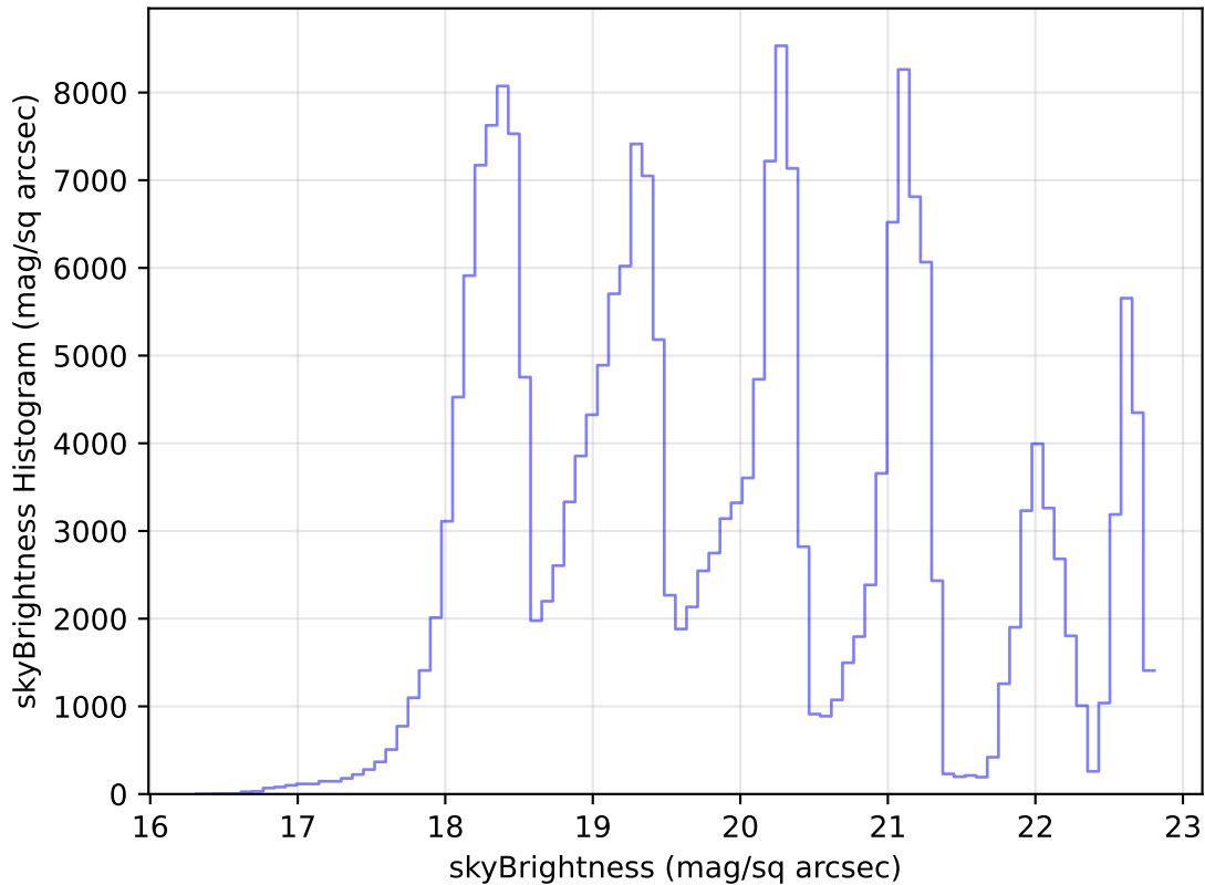
too_elab_r16_d2_griz_v3.4_10yrs Yr 1 all bands: skyBrightness Histogram
