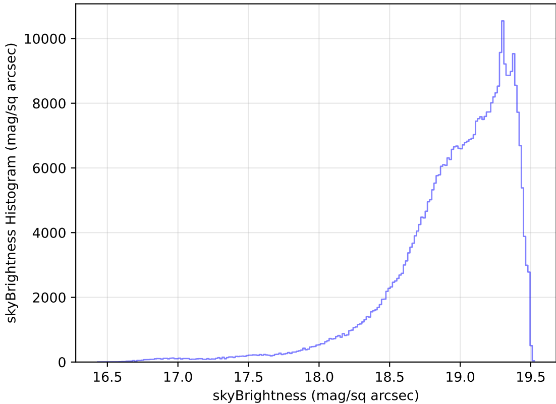
too_elab_r16_d2_griz_v3.4_10yrs WFD z band: skyBrightness Histogram
