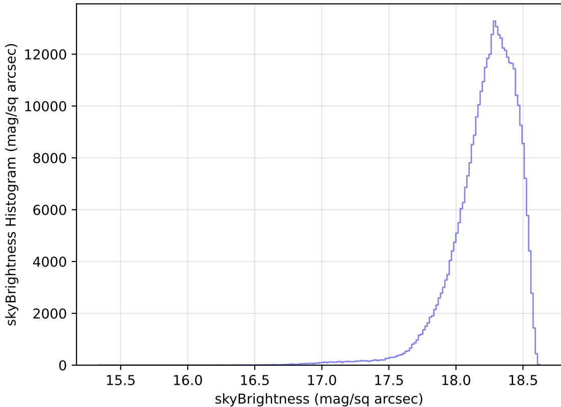
too_elab_r16_d2_griz_v3.4_10yrs WFD y band: skyBrightness Histogram
