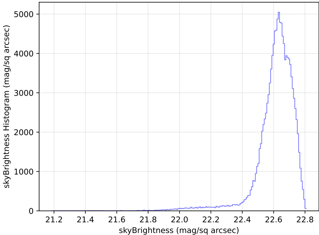
too_elab_r16_d2_griz_v3.4_10yrs WFD u band: skyBrightness Histogram
