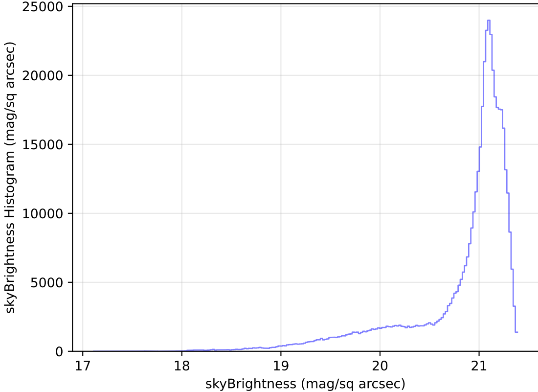
too_elab_r16_d2_griz_v3.4_10yrs WFD r band: skyBrightness Histogram
