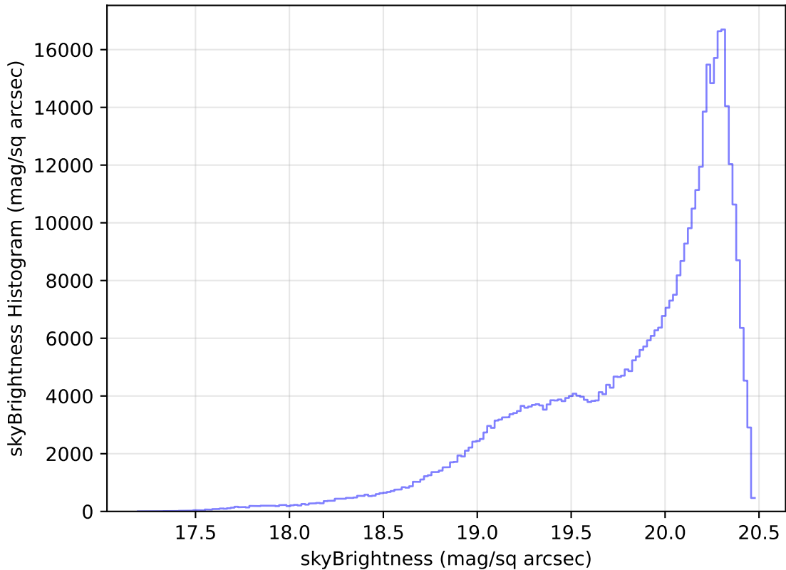
too_elab_r16_d2_griz_v3.4_10yrs WFD i band: skyBrightness Histogram
