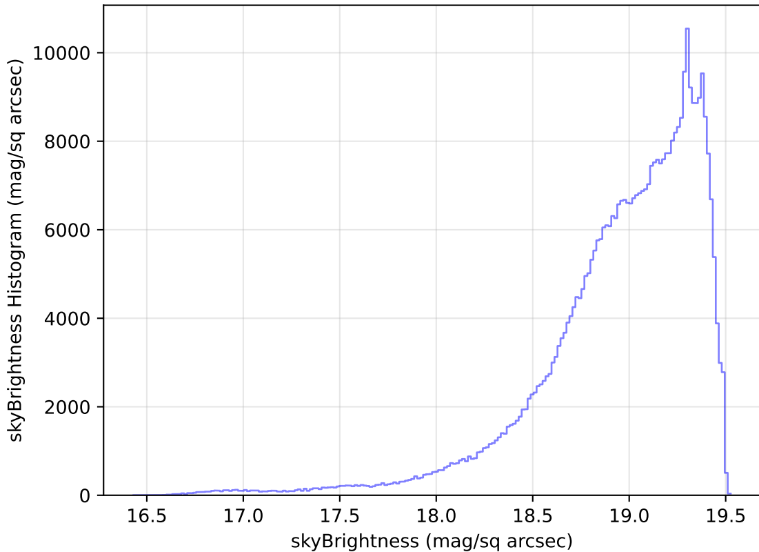
too_elab_r16_d2_griz_v3.4_10yrs All sky z band: skyBrightness Histogram
