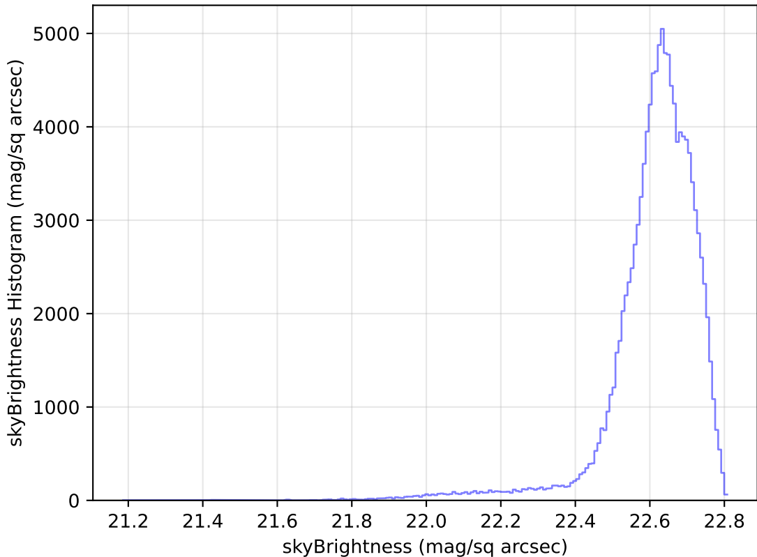
too_elab_r16_d2_griz_v3.4_10yrs All sky u band: skyBrightness Histogram
