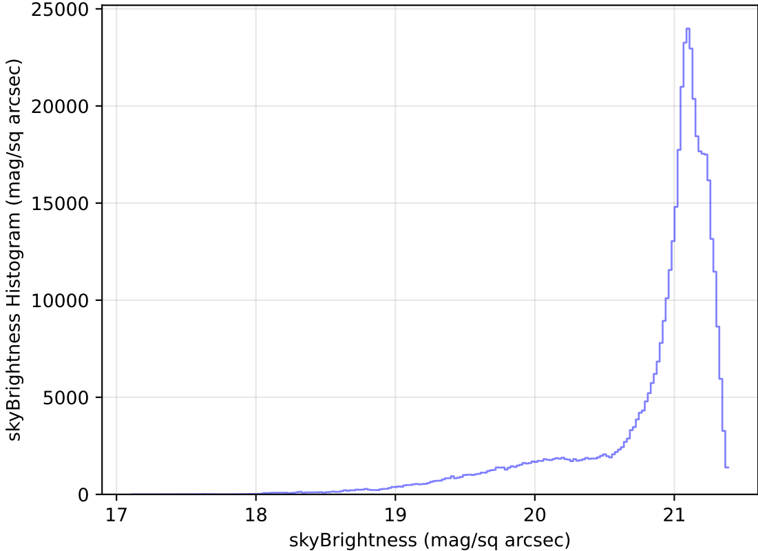
too_elab_r16_d2_griz_v3.4_10yrs All sky r band: skyBrightness Histogram
