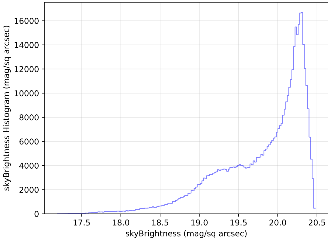
too_elab_r16_d2_griz_v3.4_10yrs All sky i band: skyBrightness Histogram
