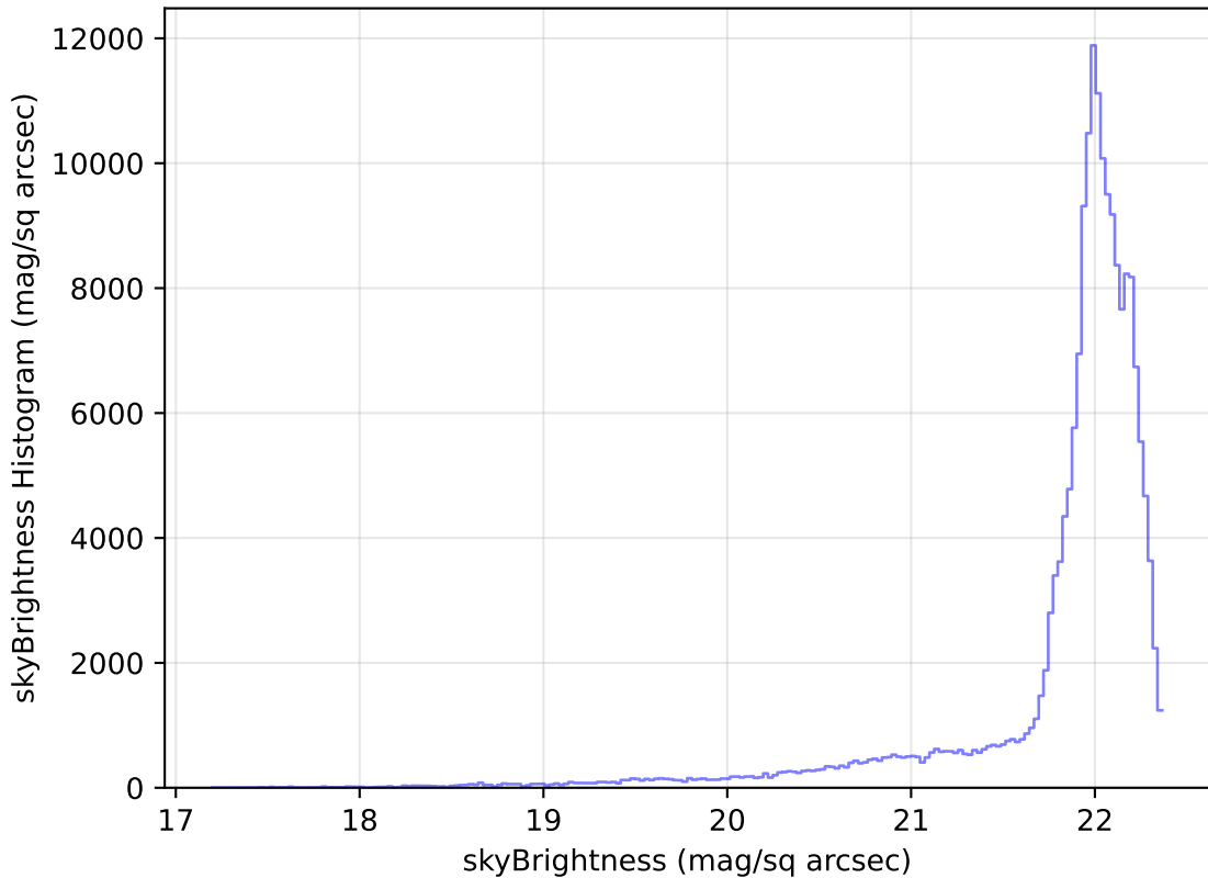
too_elab_r16_d2_griz_v3.4_10yrs All sky g band: skyBrightness Histogram
