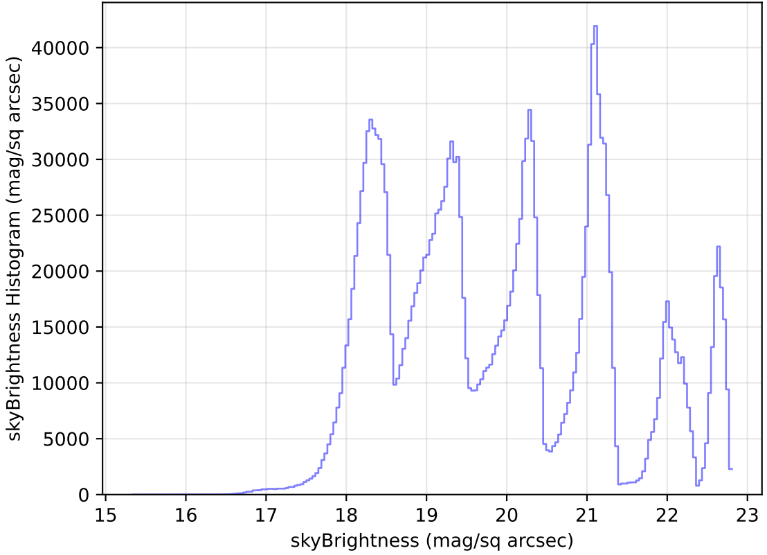
too_elab_r16_d2_griz_v3.4_10yrs All sky all bands: skyBrightness Histogram
