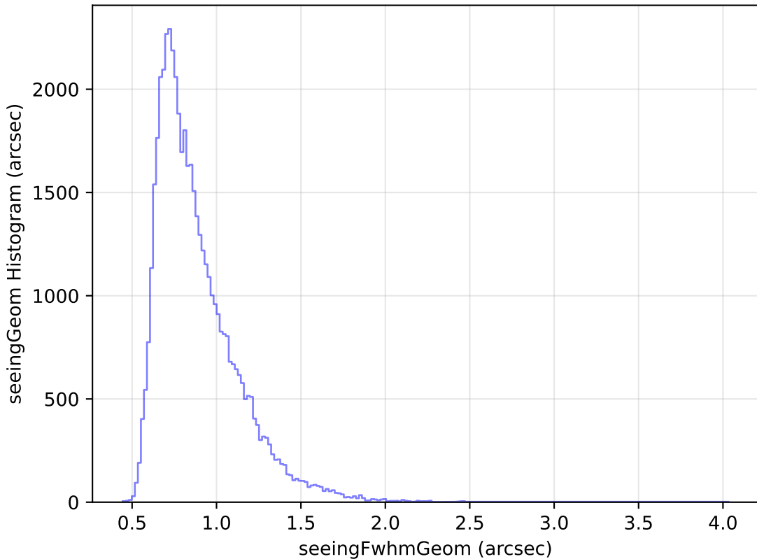
too_elab_r16_d2_griz_v3.4_10yrs Yr 1 r band: seeingGeom Histogram
