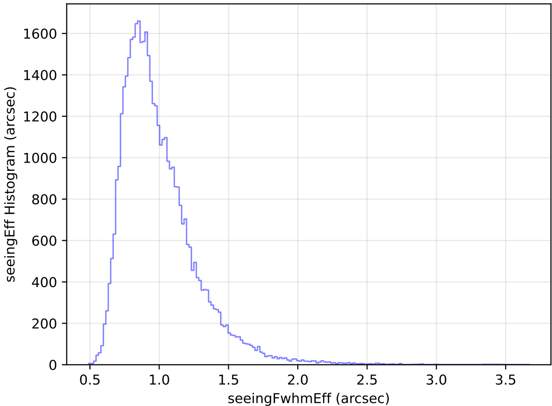
too_elab_r16_d2_griz_v3.4_10yrs Yr 1 z band: seeingEff Histogram
