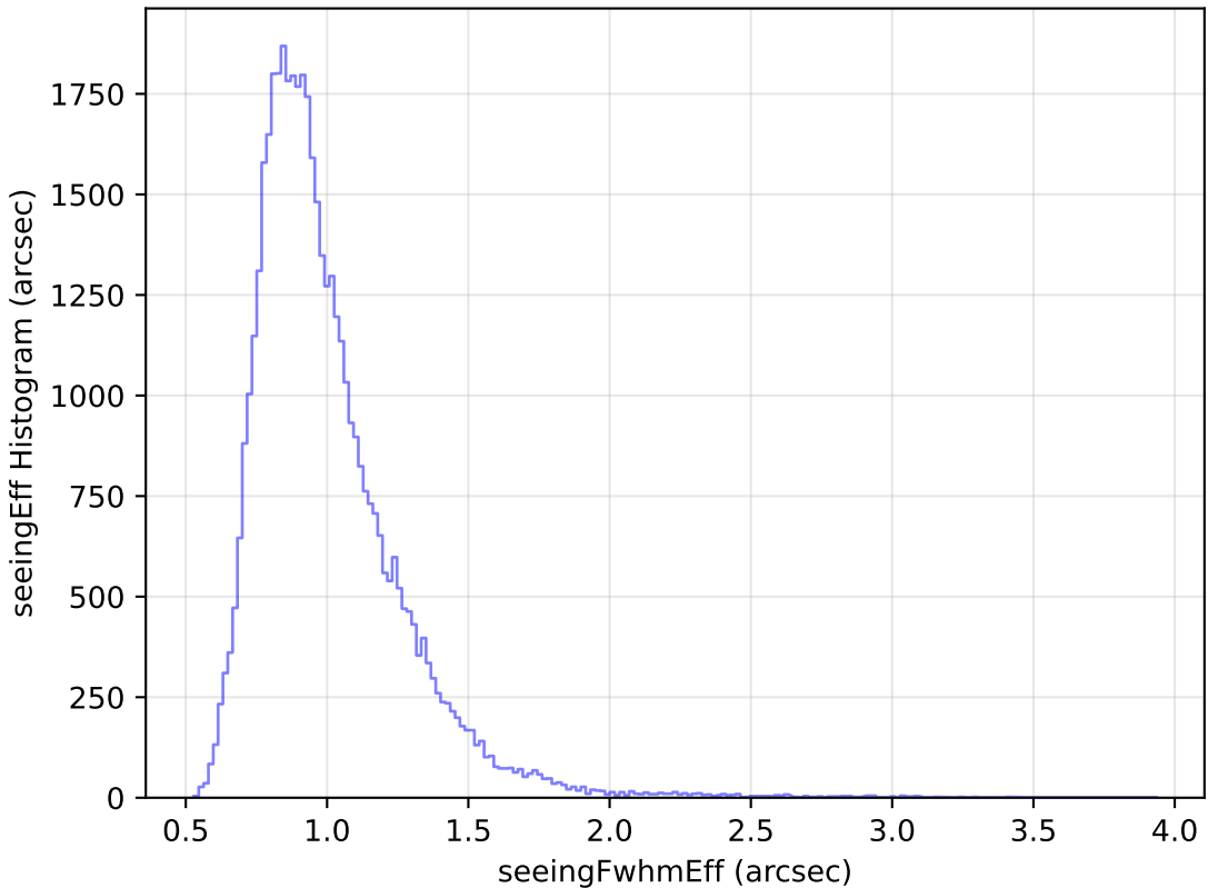
too_elab_r16_d2_griz_v3.4_10yrs Yr 1 y band: seeingEff Histogram
