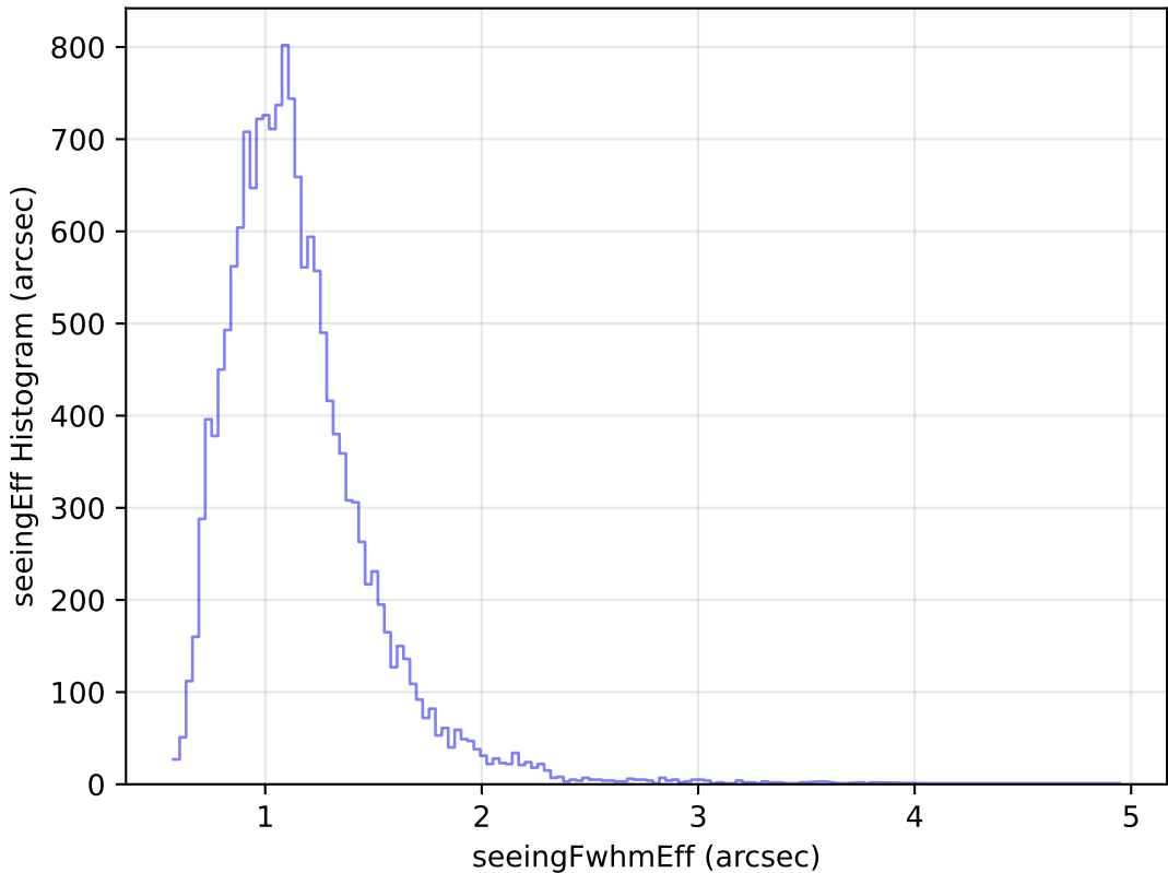
too_elab_r16_d2_griz_v3.4_10yrs Yr 1 u band: seeingEff Histogram
