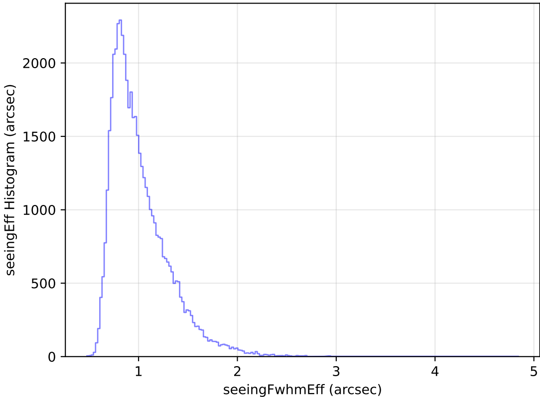
too_elab_r16_d2_griz_v3.4_10yrs Yr 1 r band: seeingEff Histogram
