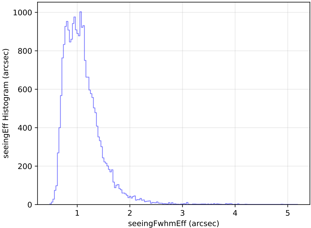
too_elab_r16_d2_griz_v3.4_10yrs Yr 1 g band: seeingEff Histogram
