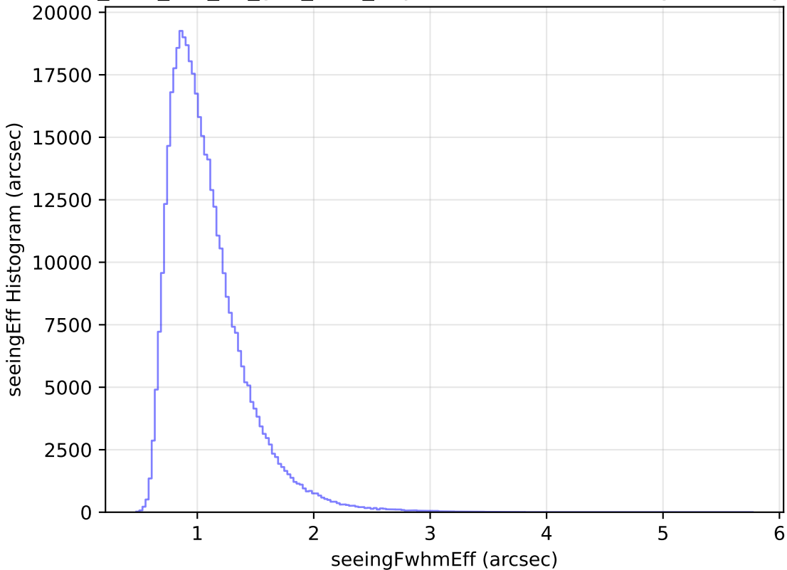
too_elab_r16_d2_griz_v3.4_10yrs WFD z band: seeingEff Histogram
