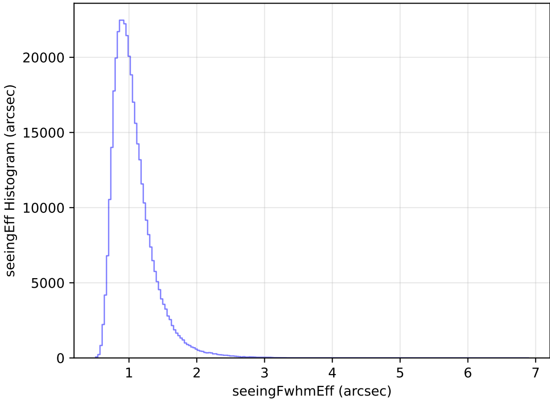
too_elab_r16_d2_griz_v3.4_10yrs WFD y band: seeingEff Histogram
