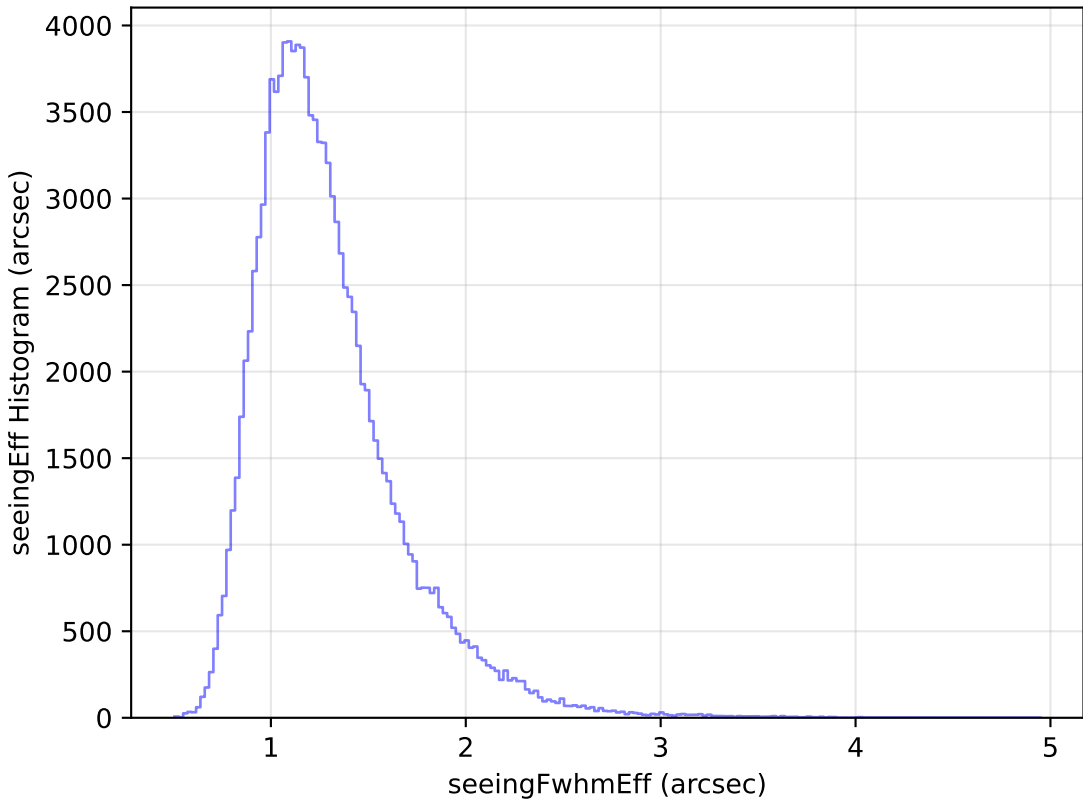
too_elab_r16_d2_griz_v3.4_10yrs WFD u band: seeingEff Histogram
