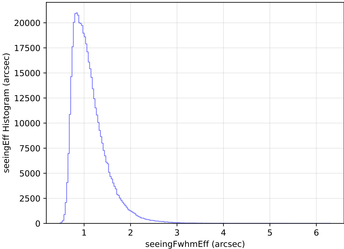
too_elab_r16_d2_griz_v3.4_10yrs WFD r band: seeingEff Histogram
