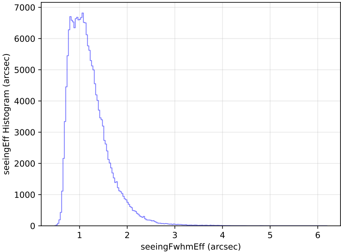
too_elab_r16_d2_griz_v3.4_10yrs WFD g band: seeingEff Histogram
