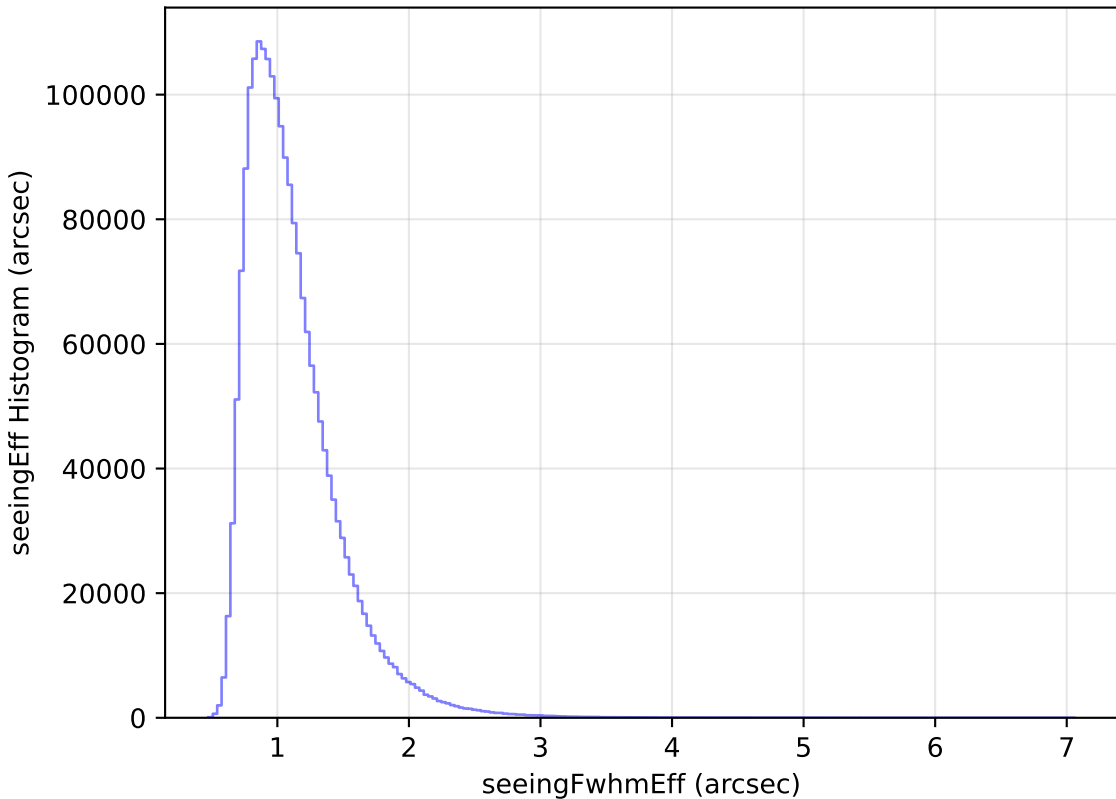
too_elab_r16_d2_griz_v3.4_10yrs WFD all bands: seeingEff Histogram
