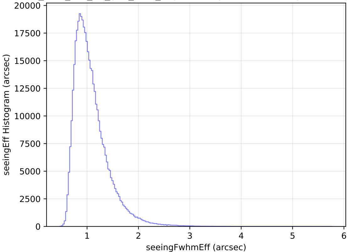
too_elab_r16_d2_griz_v3.4_10yrs All sky z band: seeingEff Histogram
