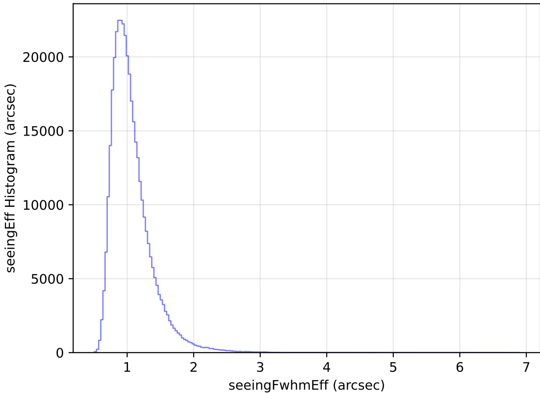
too_elab_r16_d2_griz_v3.4_10yrs All sky y band: seeingEff Histogram
