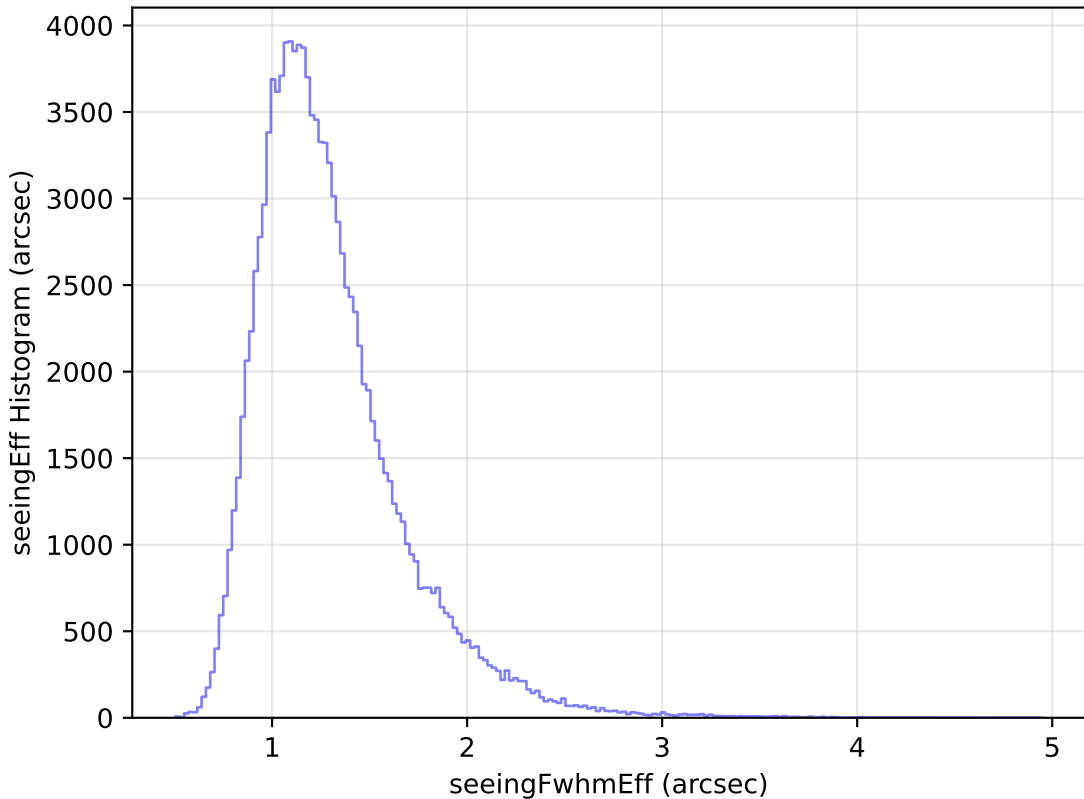
too_elab_r16_d2_griz_v3.4_10yrs All sky u band: seeingEff Histogram
