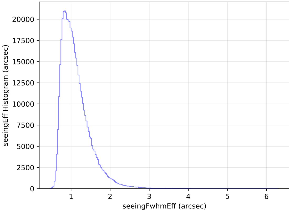
too_elab_r16_d2_griz_v3.4_10yrs All sky r band: seeingEff Histogram
