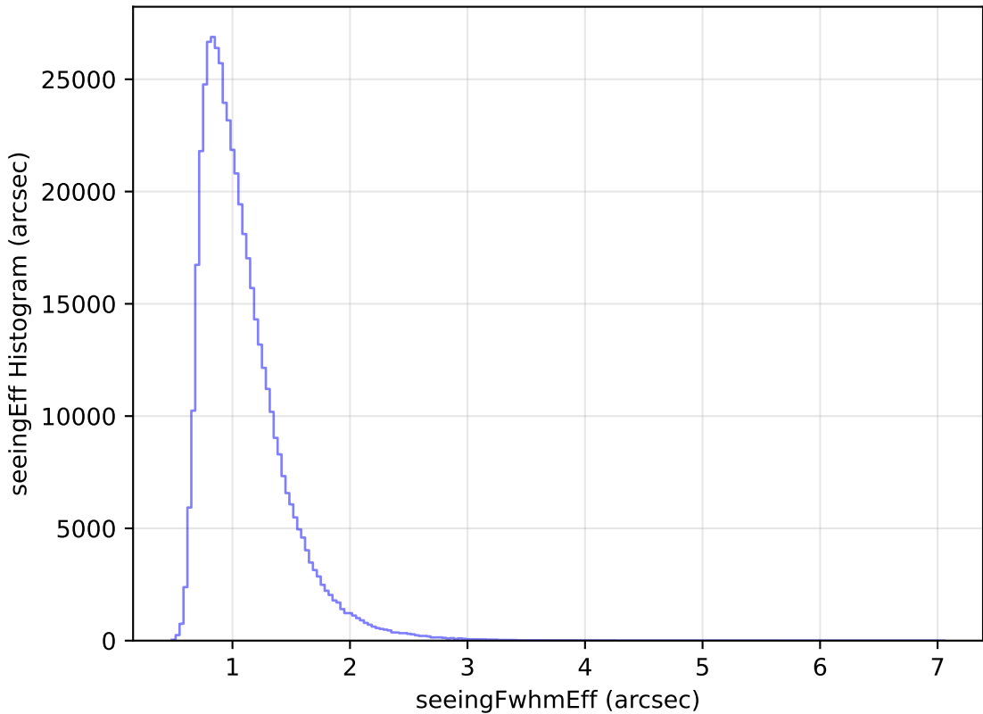
too_elab_r16_d2_griz_v3.4_10yrs All sky i band: seeingEff Histogram
