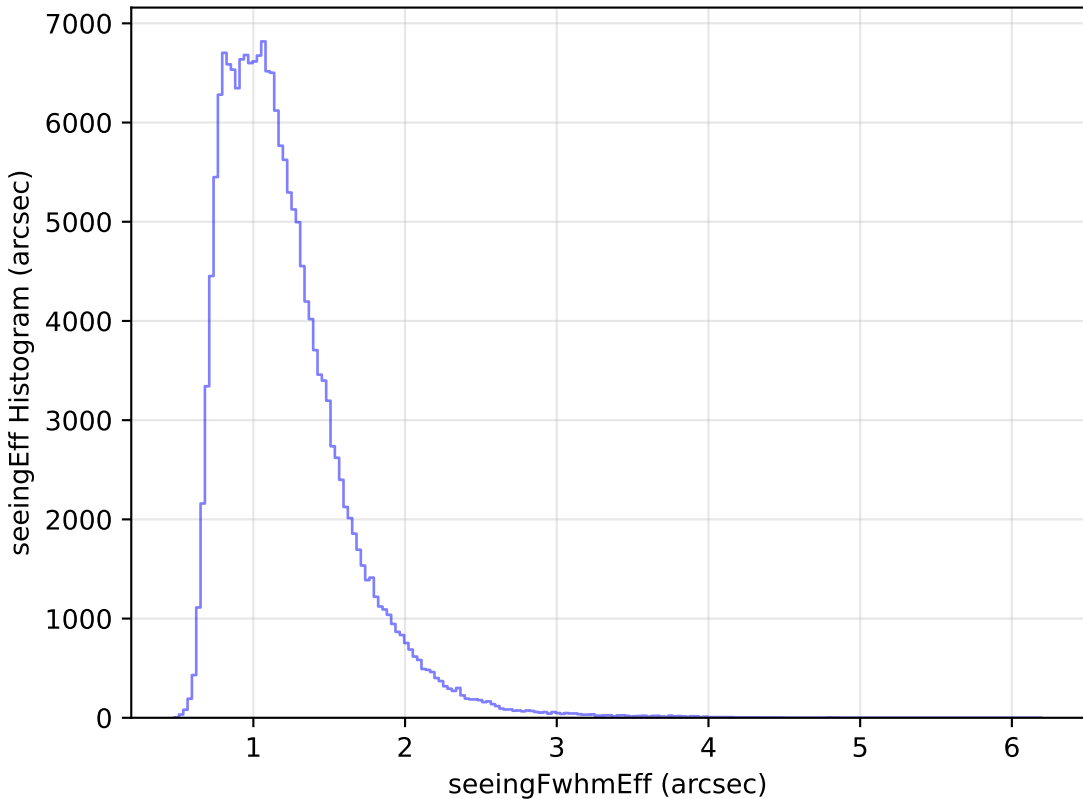
too_elab_r16_d2_griz_v3.4_10yrs All sky g band: seeingEff Histogram
