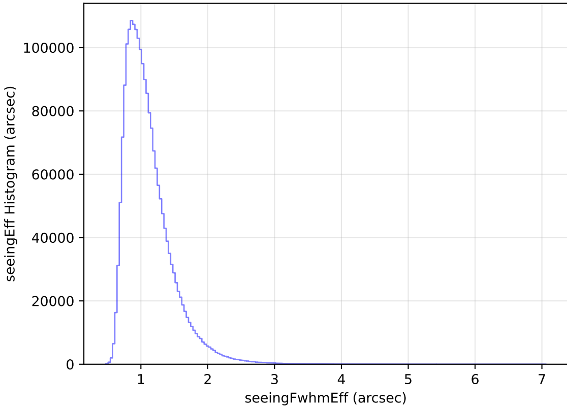
too_elab_r16_d2_griz_v3.4_10yrs All sky all bands: seeingEff Histogram
