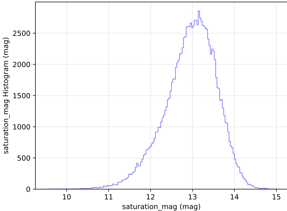
too_elab_r16_d2_griz_v3.4_10yrs WFD u band: saturation_mag Histogram
