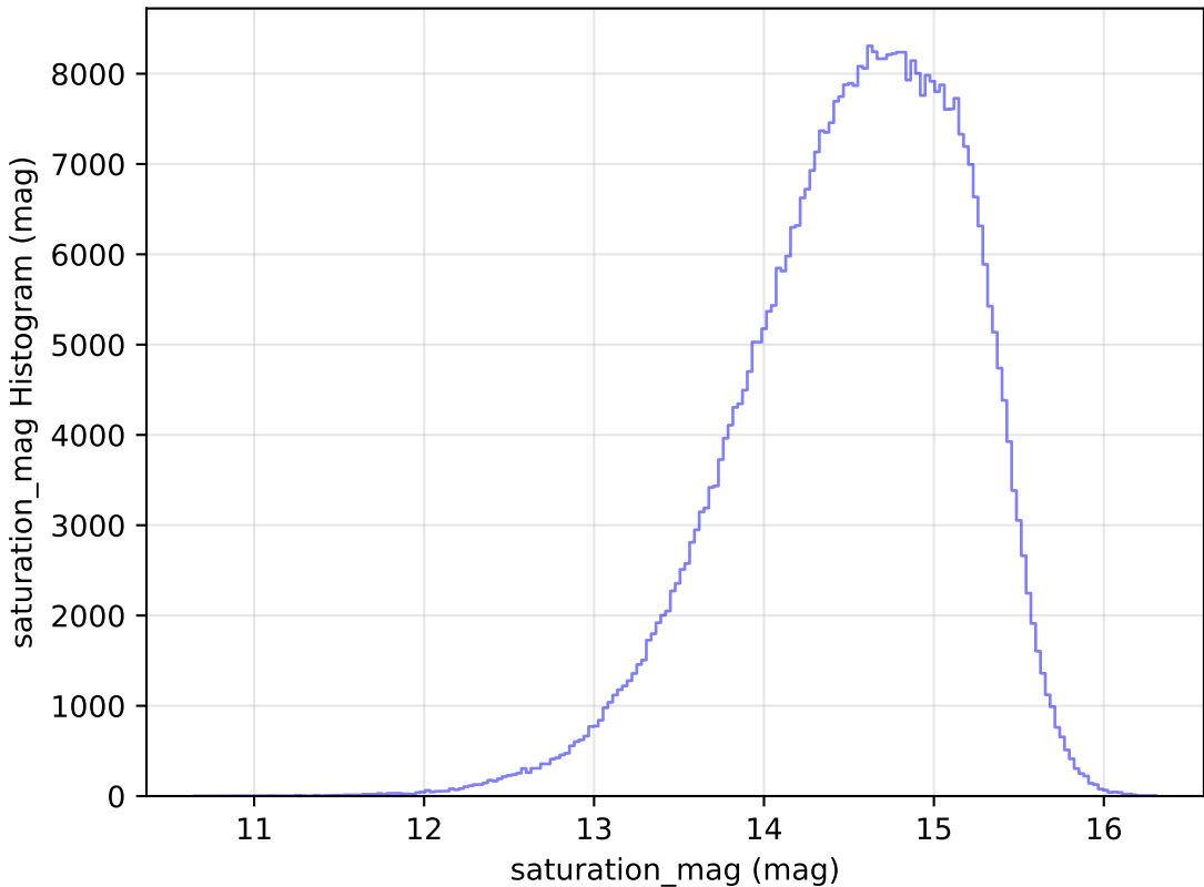
too_elab_r16_d2_griz_v3.4_10yrs WFD r band: saturation_mag Histogram
