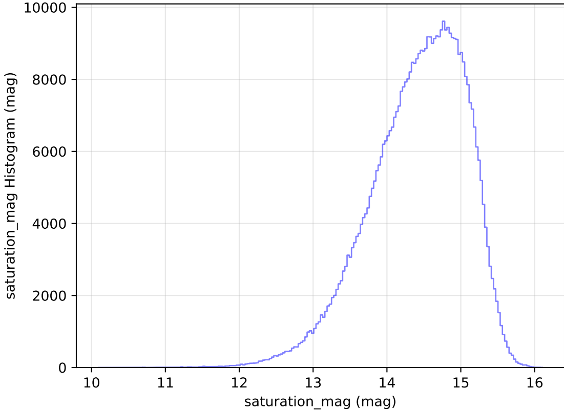
too_elab_r16_d2_griz_v3.4_10yrs WFD i band: saturation_mag Histogram
