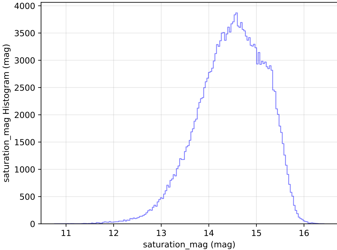
too_elab_r16_d2_griz_v3.4_10yrs WFD g band: saturation_mag Histogram
